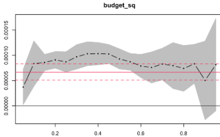
Figure 6. The impact of film revenue on budget square along quantile levels of budget square.
