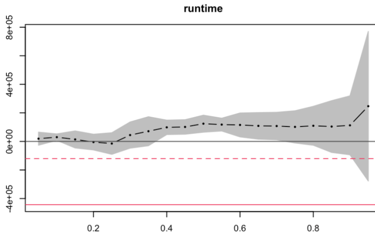
Figure 3. The impact of film revenue on runtime along quantile levels of runtime.
